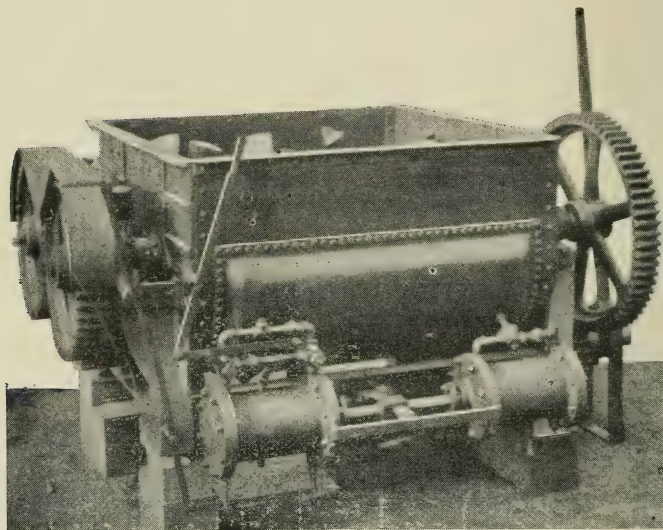
FIG. 117.—Mixer for Preparing Paving Compositions.
